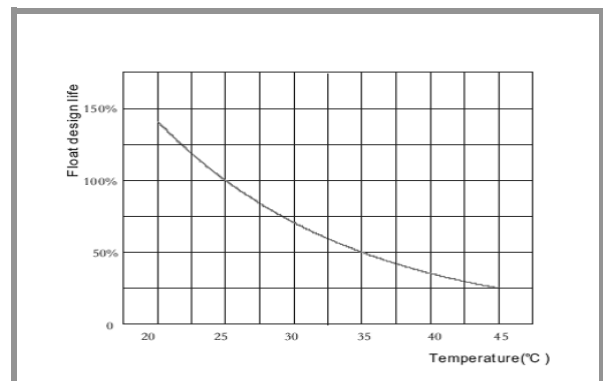
Temperature Vs. design Life Curve
