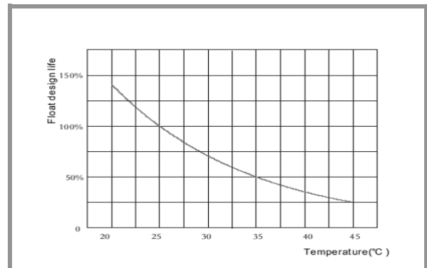
Temperature Vs. design Life Curve
