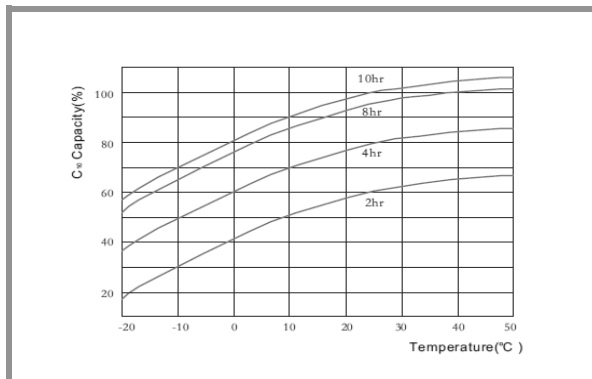
Temperature Vs. Capacity Curve
